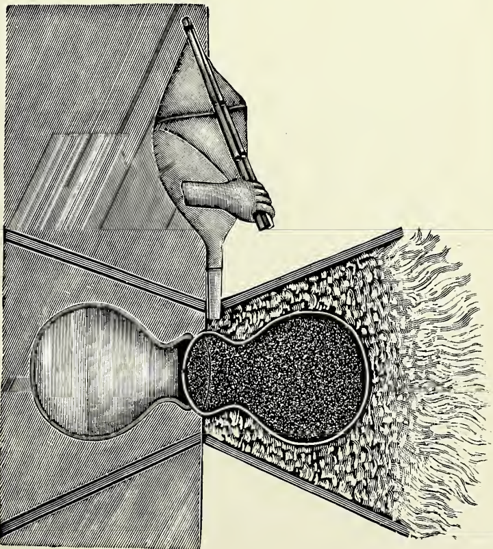
Kosh hi apparatus, for the extraction of zinc from calamine. (See p. 89)
